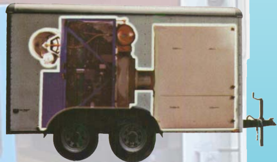
Trailer Mounted Air Duct Cleaning Setup (Recommended Trailer - 6' x 12' Tandem Axle Trailer)
